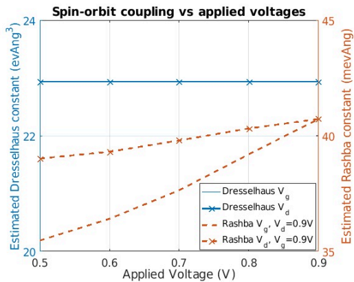
FIG. 12. Dependence of Rashba and Dresselhaus coupling on source-drain and gate voltage.
